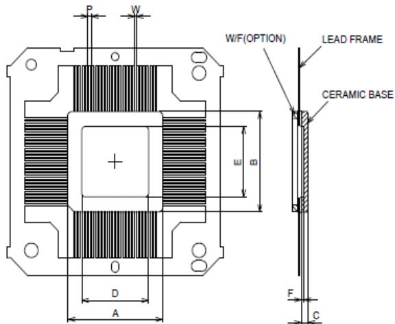
FLAT LEAD
