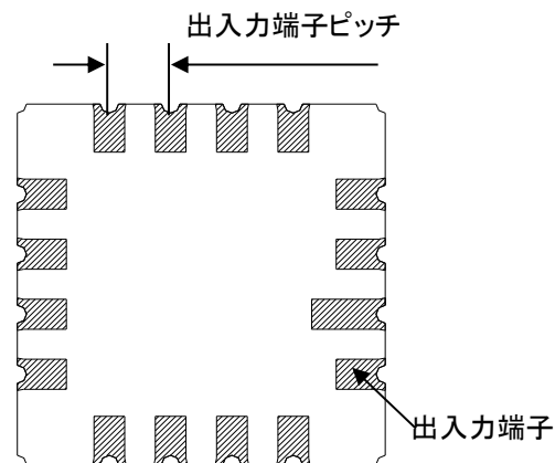
Leadless Chip Carrier (LCC) = Quad Flat No Lead (QFN)
