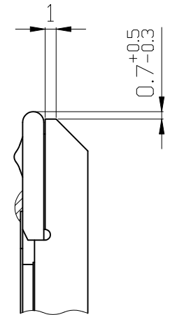
MAGNIFIED VIEW OF PART "A" (2/1)
